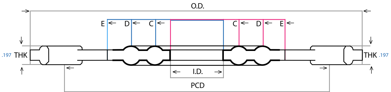
APPROXIMATE DIMENSIONS
