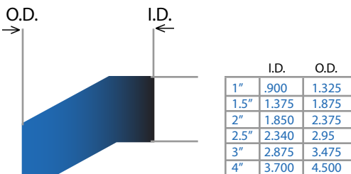
CROSS SECTION PROFILE - APPROXIMATE DIMENSIONS
