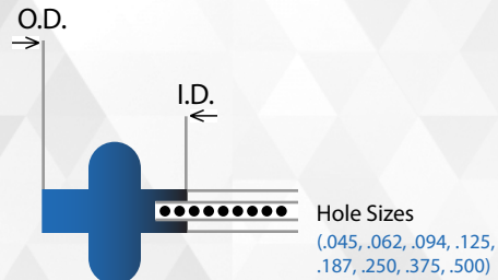
CROSS SECTION PROFILE - APPROXIMATE DIMENSIONS
